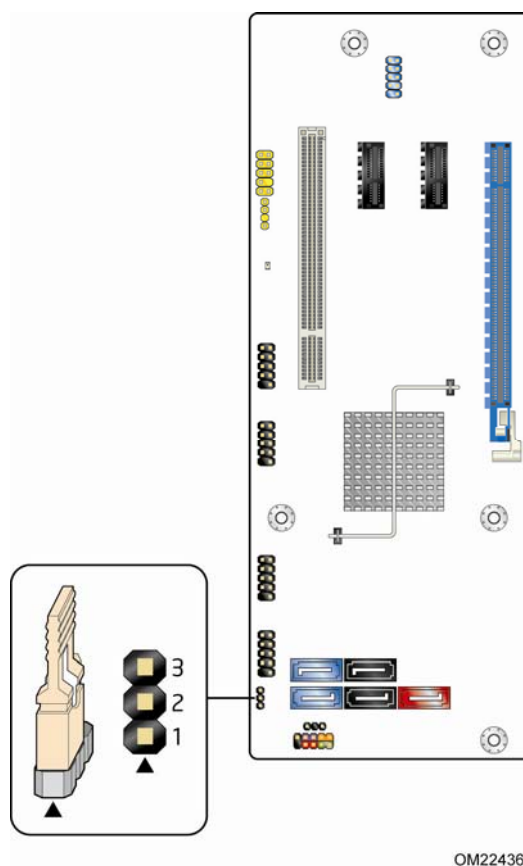
Figure 13. Location of the Jumper Block
