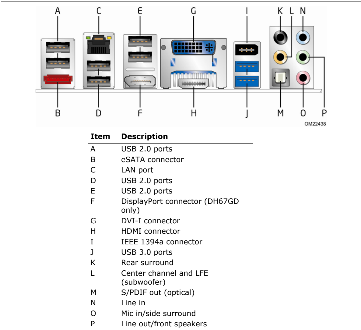
Figure 9. Back Panel Connectors
