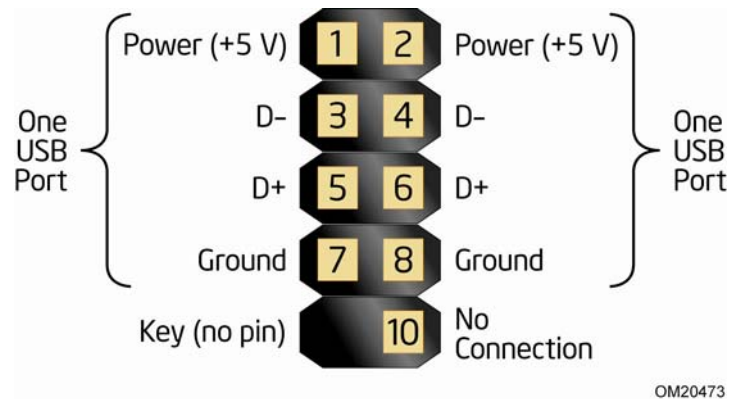
Figure 12. Connection Diagram for Front Panel USB 2.0 Headers
